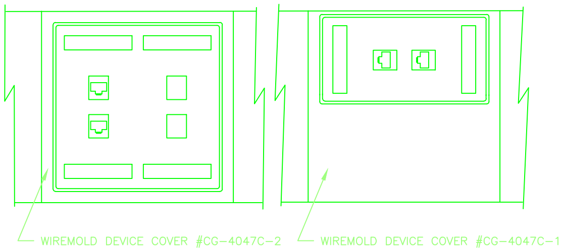
COMMUNICATIONS OUTLET MOUNTED ON G-4000 OR G-6000 WIREMOLD – TYPICAL
