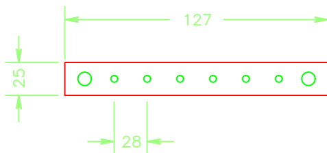
BUS BAR FOR ENTRANCE FACILITIES GROUND
