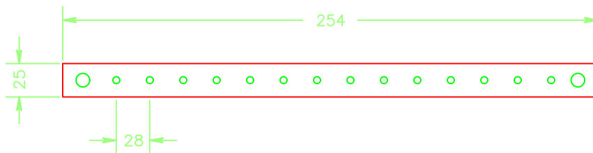
GROUND BUS BAR IN LOCAL COMMUNICATIONS ROOMS (TGB)
