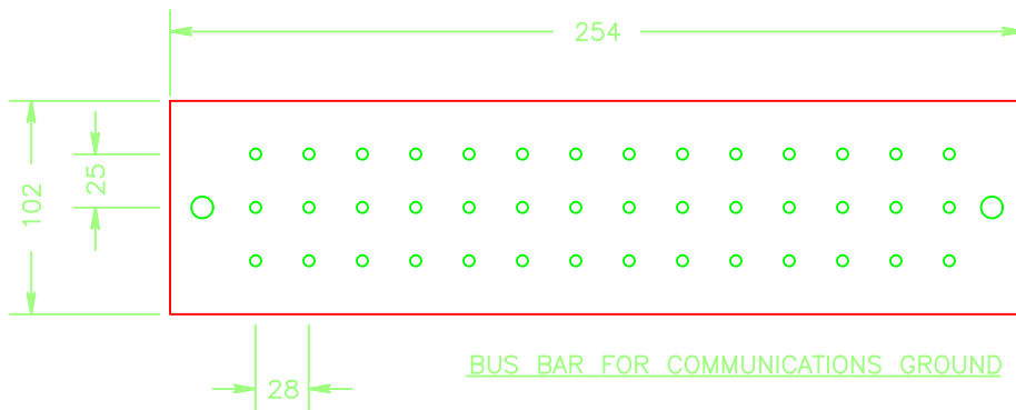
GROUND BUS BAR IN MAIN COMMUNICATIONS ROOM (TMGB)
